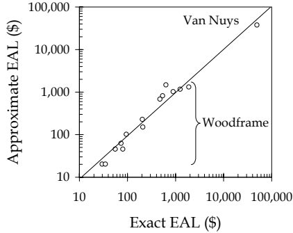
Figure 3. Comparing EAL by methods 1 and 2 for 15 sample buildings
