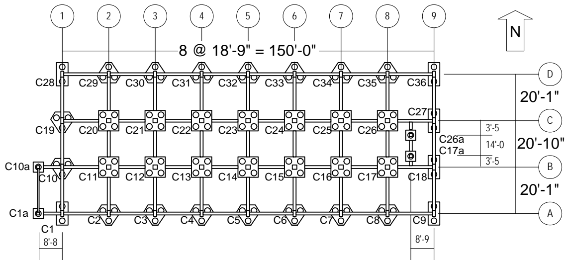
Figure 4. Foundation and column plan, showing designer's notation for column numbers.
