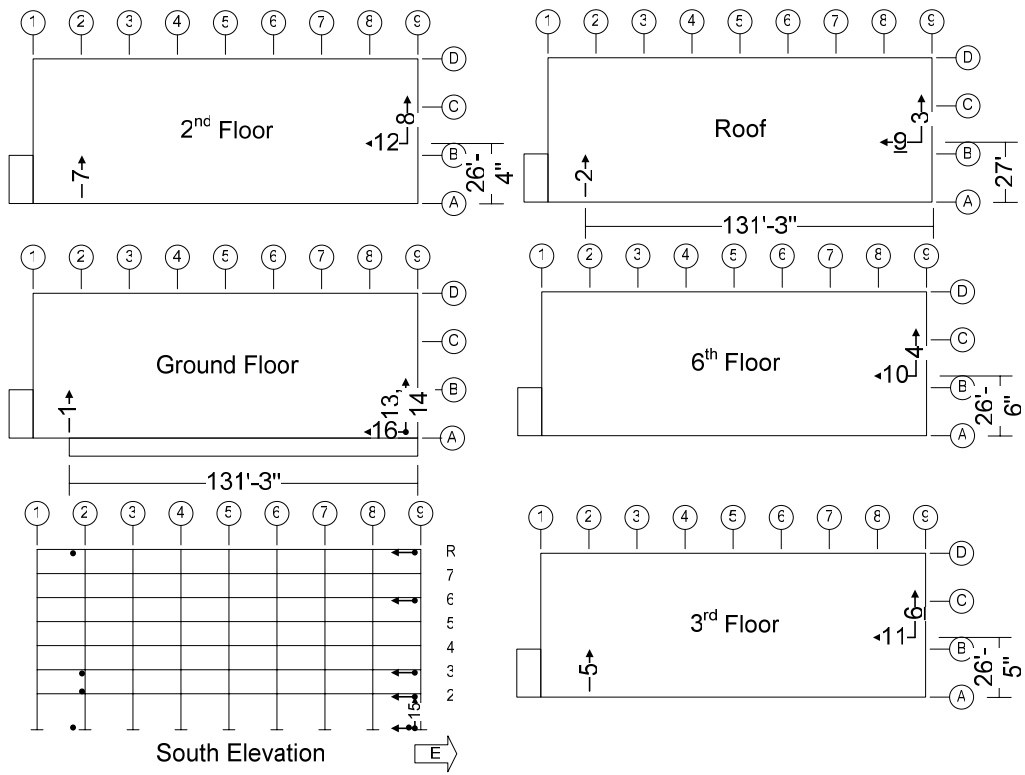
Figure 6. Instrument locations after 1980
