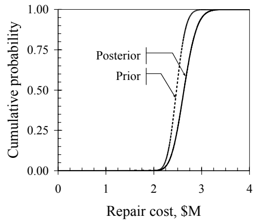
Figure 7. Hindcast repair cost distributions for the 1994 Northridge earthquake. Posterior uses upper-story sensor data.
