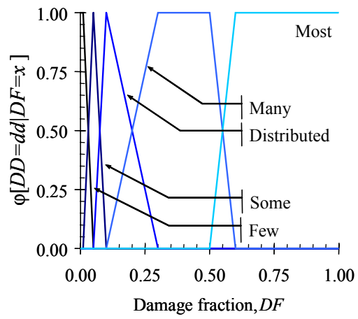
Figure 3. Membership functions relating damage description to damage fraction
