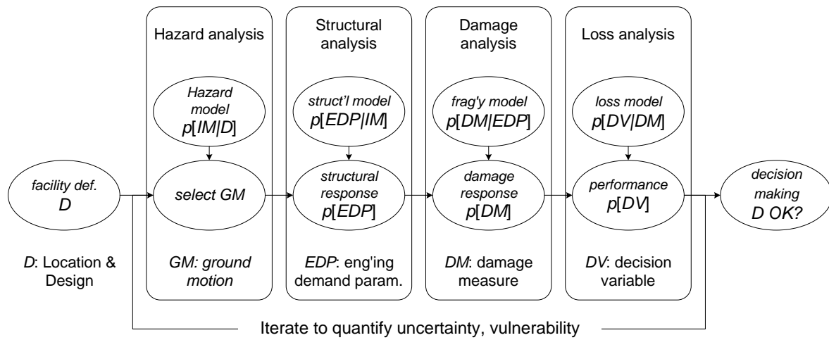
Figure 1. Framework of probabilistic PBEE methodologies
