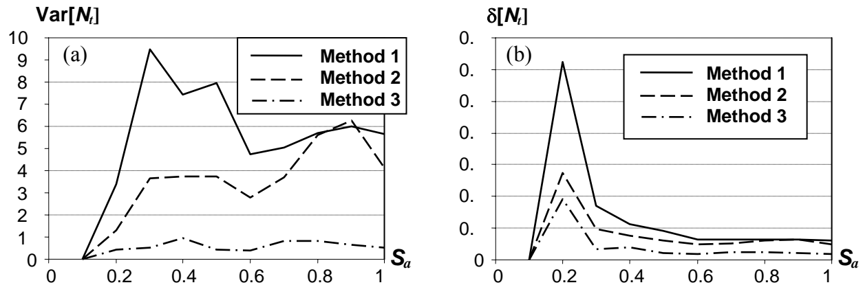
Figure 7. Variance of the damage estimate (a) and coefficient of variation (b), ground motion LA15.
