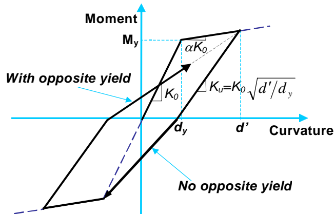
Figure 5. Flexural members hysteretic rule: Q-HYST.
