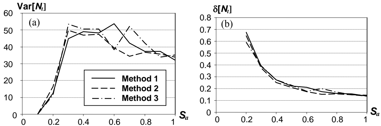
Figure 9. Variance of damage estimation (a) and coefficient of variation (b), set of ground motions.
