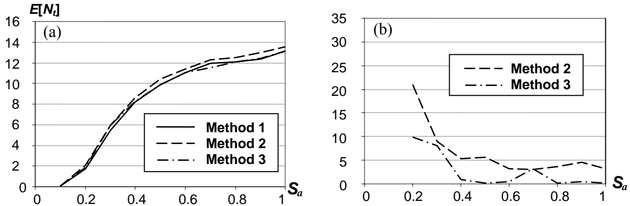
Figure 8. Expectation of damage (a) and relative difference (b), set ground motions.
