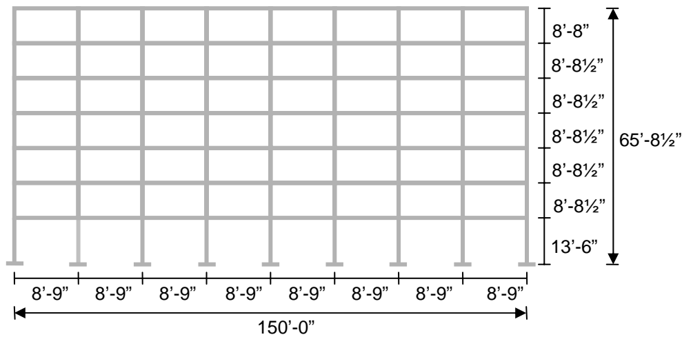
Figure 4. Reinforced concrete moment-resisting frame chosen for the case study.
