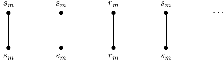
FIGURE 5: The comb s_m^2
