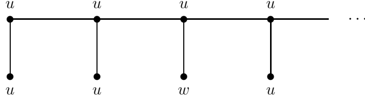
FIGURE 3: The comb u^2
