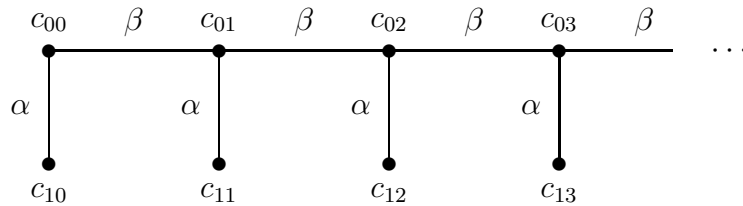
FIGURE 2: The ‘‘comb’’ (c_{0j}, c_{1j})_{j < \kappa}
