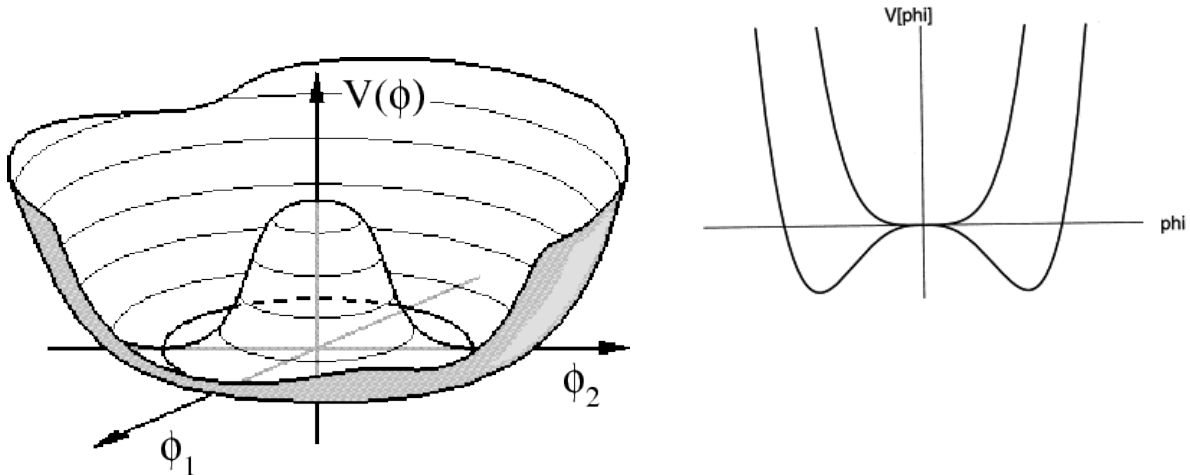
FIG. 6: A Mexican-hat potential and its cross-section controlling a continuous phase transition, illustrated for a two component order parameter \Phi = (\phi_1, \phi_2) (e.g., the normal-to-superfluid or XY PM-FM). Massive (gapped) amplitude (Higg’s) and gapless Goldstone mode excitations respectively correspond to radial and azimuthal fluctuations about \Phi_0 .
